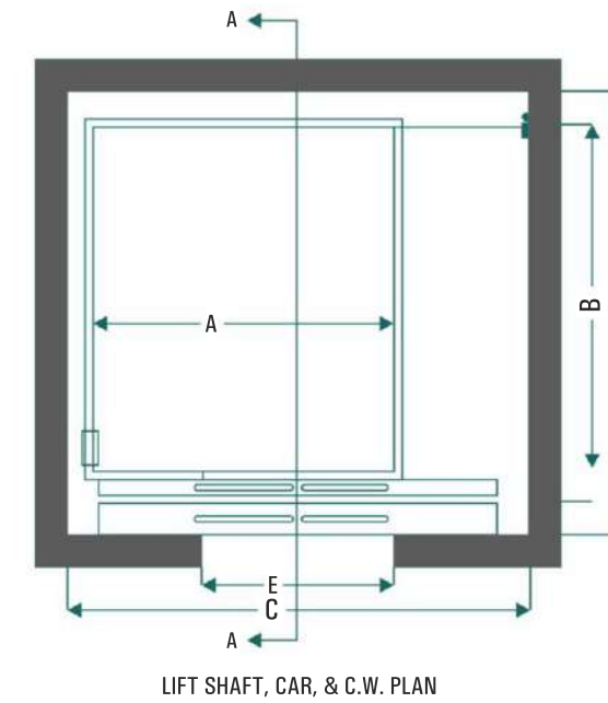
LIFT SHAFT, CAR, & C.W. PLAN
