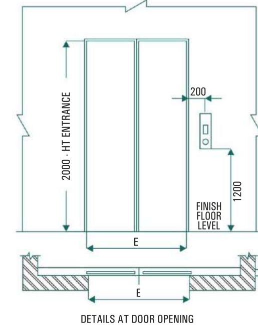
DETAILS AT DOOR OPENING
