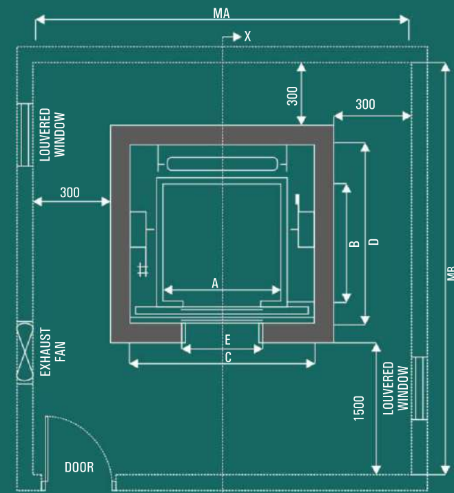
LIFT SHAFT, CAR, C.W. & MACHINE ROOM PLAN
