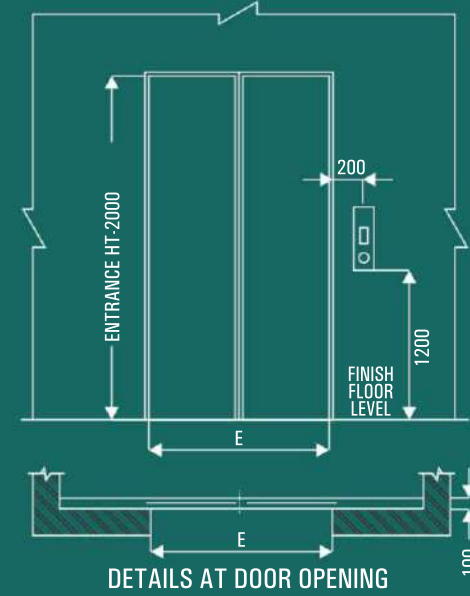
DETAILS AT DOOR OPENING
